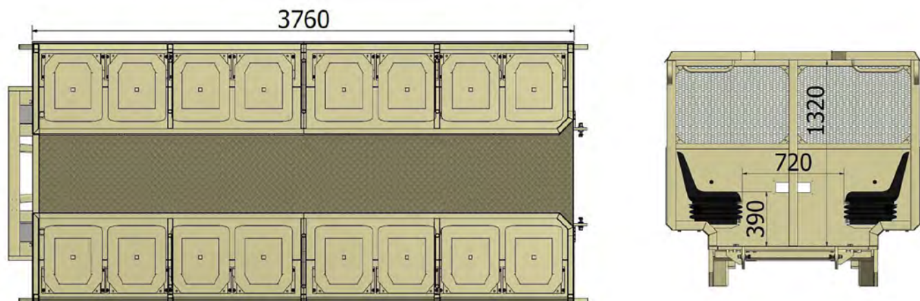
Seat layout for top and inside view
