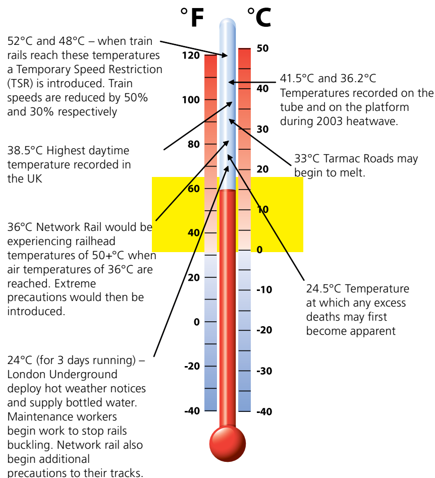
Figure 4. Trigger temperatures
