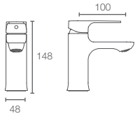
FORE TRI™ | K-27477IN-4ND-CP
