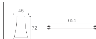
COMPLEMENTARY™ | K-5630IN-CP 610mm towel bar in polished chrome
