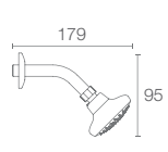
COMPLEMENTARY™ K-16356IN-A-CP Single-function showerhead in polished chrome (with shower arm and flange)
