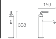
Purist™* | K-14404IN-4AND-BL Tall single-control lavatory faucet with straight lever handle without drain
