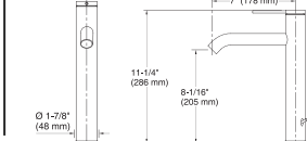
Components™* | K-77959-4A-BL Single-handle bathroom sink faucet
