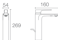
Aleo+™ | K-72337IN-4ND-BL Tall lavatory faucet without drain
