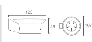
Accent™ | K-25429IN-BL Soap Dish
