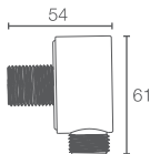
Complementary™ | K-22448IN-BL Supply Elbow
