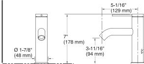
Components™* | K-77958-4A-BL Single-handle bathroom sink faucet
