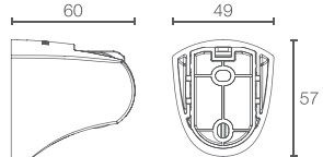
Complementary™ | K-99035IN-BL Handshower Bracket
