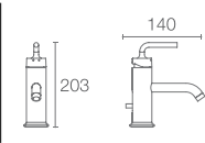
Purist™* | K-14402-4A-BL Single-handle bathroom sink faucet with straight lever handle
