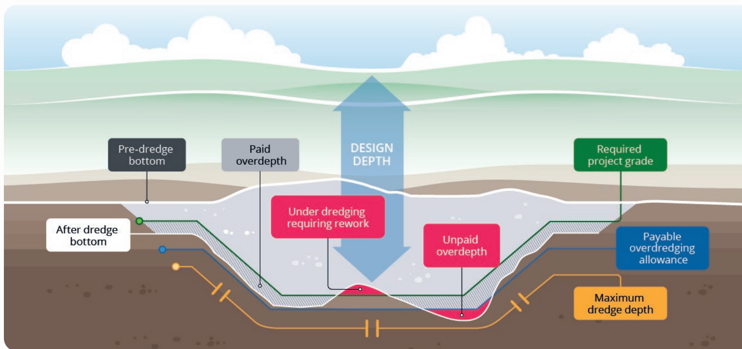
Figure 1. Various Dredging prism dimensions and zones.
