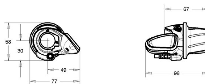
H8 Controller
