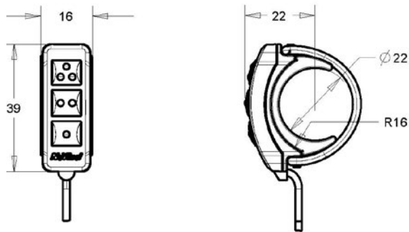
H3 controller
