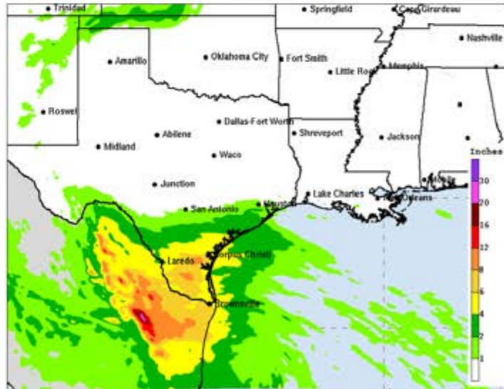
Potential Tropical Cyclone One Day 1-2 Rainfall Forecast (inches) Created 2:00 AM CDT Wed Jun 19 2024 Valid 1:00 AM CDT Wed Jun 19 2024 through 7:00 AM CDT Fri Jun 21 2024 DOC:NOAA/NWS/NCEP/WPC Local point maximum rainfall may be higher than shown. See the NHC public advisories for the latest tropical cyclone information.
