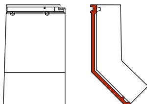
knikgevelpan links 140°
