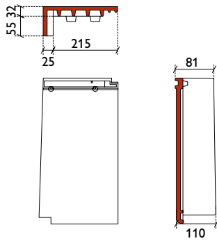
gevelpan links
