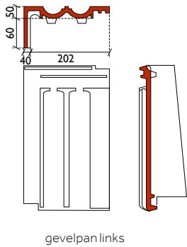
gevelpan links
