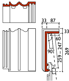
chaperonpan 90°
