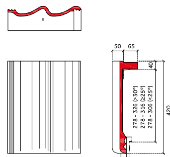
chaperonpan 90°
