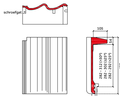
chaperonpan 90°
