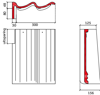
gevelpan links
