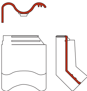
knikgevelpan links 140°
