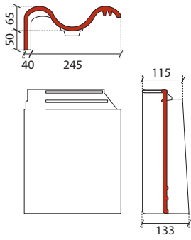
gevelpan links
