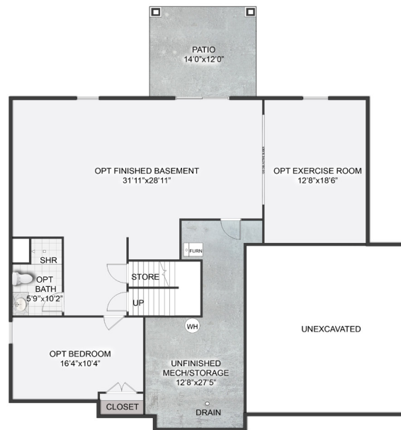
OPT LUXURY REAR WALKOUT FOUNDATION PLAN
