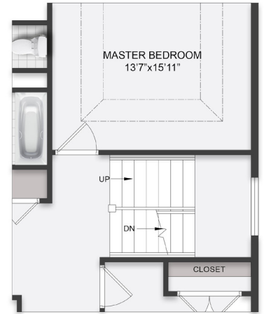
SECOND FLOOR PARTIAL PLAN
