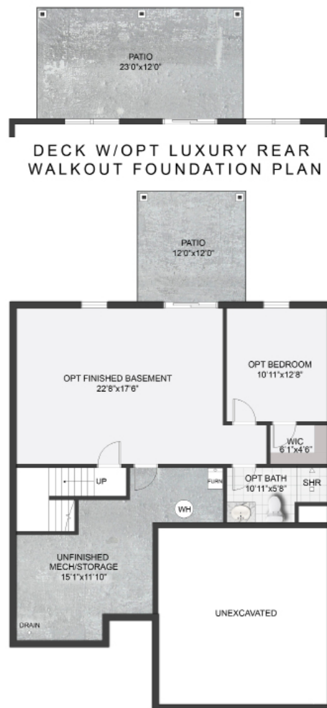
OPT SIGNATURE REAR WALKOUT FOUNDATION PLAN W/OPT FINISHED BASEMENT
