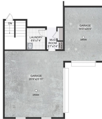
OPT. 3 CAR SPLIT ENTRY GARAGE
