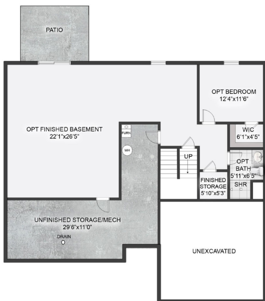
OPT. LUXURY REAR WALKOUT FOUNDATION PLAN
