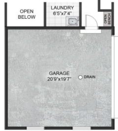
OPT. 2 CAR SPLIT ENTRY GARAGE
