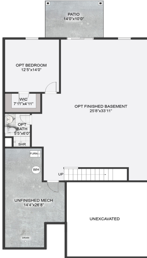
REAR WALKOUT FOUNDATION PLAN
