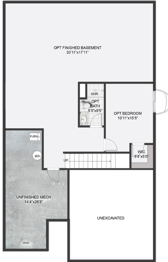
BURIED FOUNDATION PLAN W/ OPT FINISHED BASEMENT
