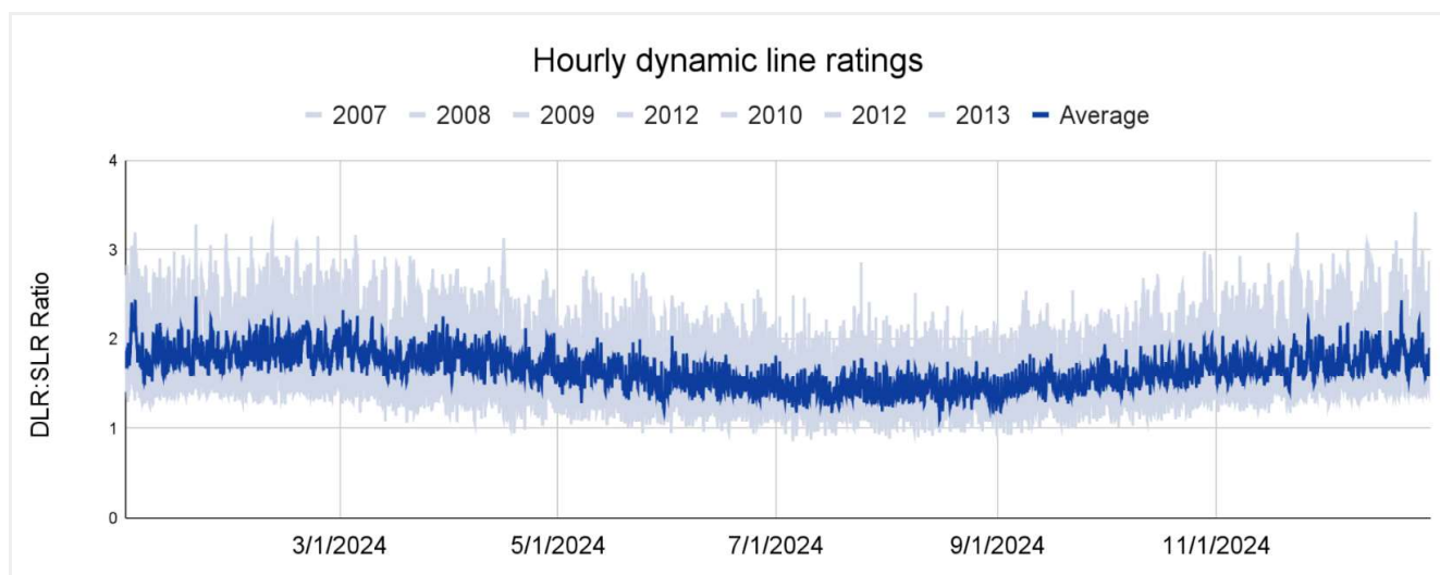
Figure 21: Ratio of Dynamic Line Rating to Standard Line Rating for One-Year Period
