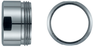
M20 Ø Thread connection: ~19 mm Ø Sieb: ~20 mm
