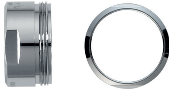
M24 Ø Thread connection: ~23 mm Ø Bottom side: ~24 mm
