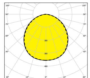
— C0-C180 - - - - C90-C270
