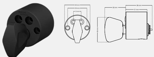
Vrider cylinder KC2573SL
