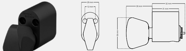
Vrider cylinder KC2542SL
