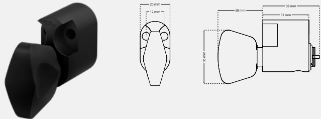
Vrider cylinder KC2549SL
