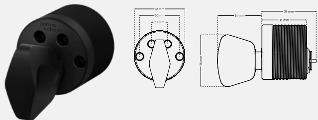
Vrider cylinder KC2572SL
