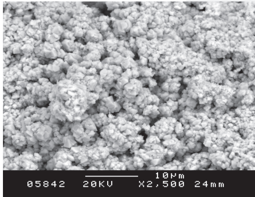
Figure 2: Structure of Trojan's OverDrive Battery Plate
