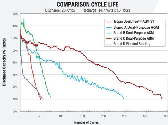
Figure 1: OverDrive Outperforms Other Battery Types
