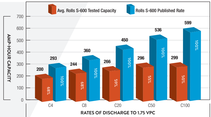
TESTED AND PUBLISHED CAPACITIES FOR THE ROLLS S-600 BATTERY**
