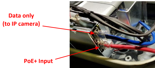
Fig 19 CHAT™ board, showing PoE+ (802.3at) input & data output
