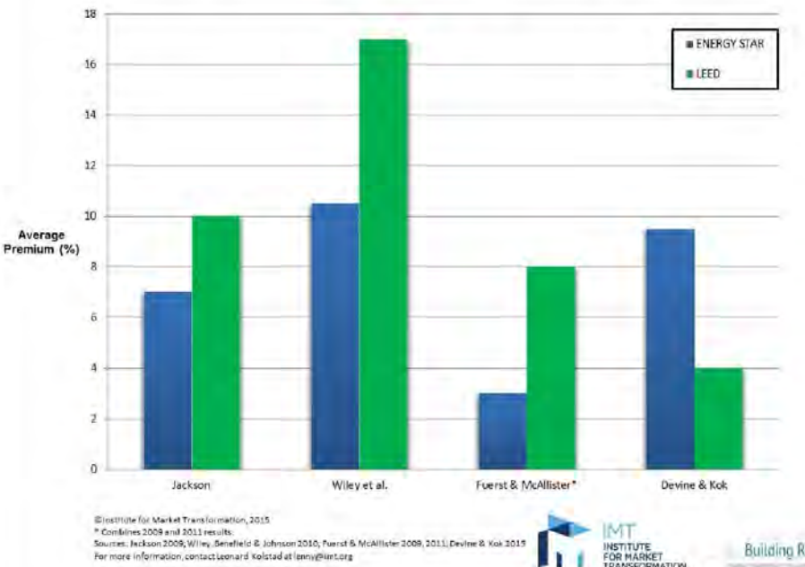
Figure 5b. Occupancy premiums of green buildings. (IMT 2016)
