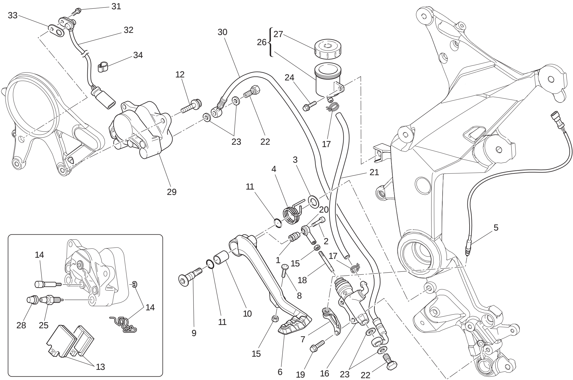
DRAWING 025 Rear brake
