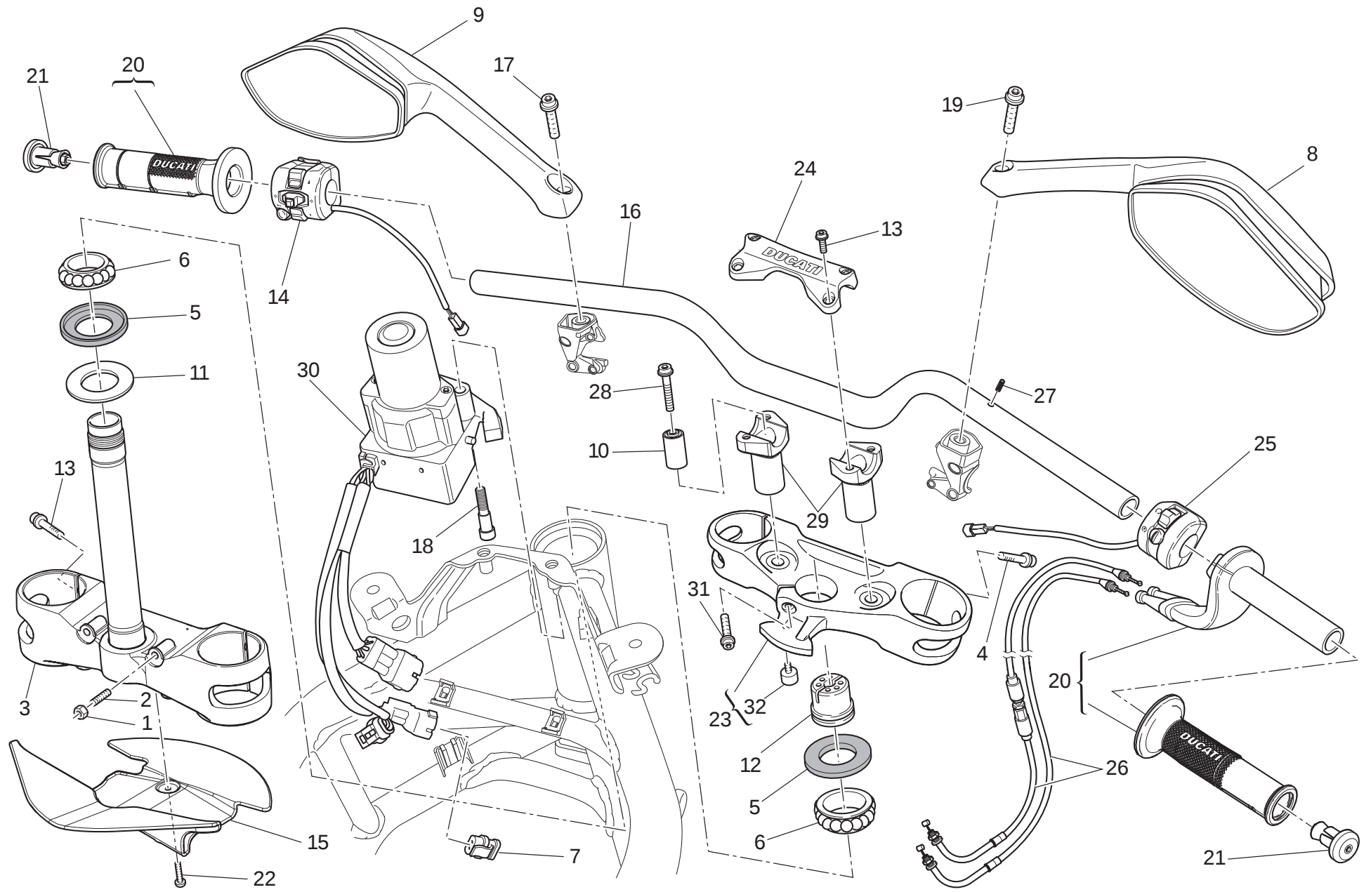
DRAWING 021 Handlebar and controls
