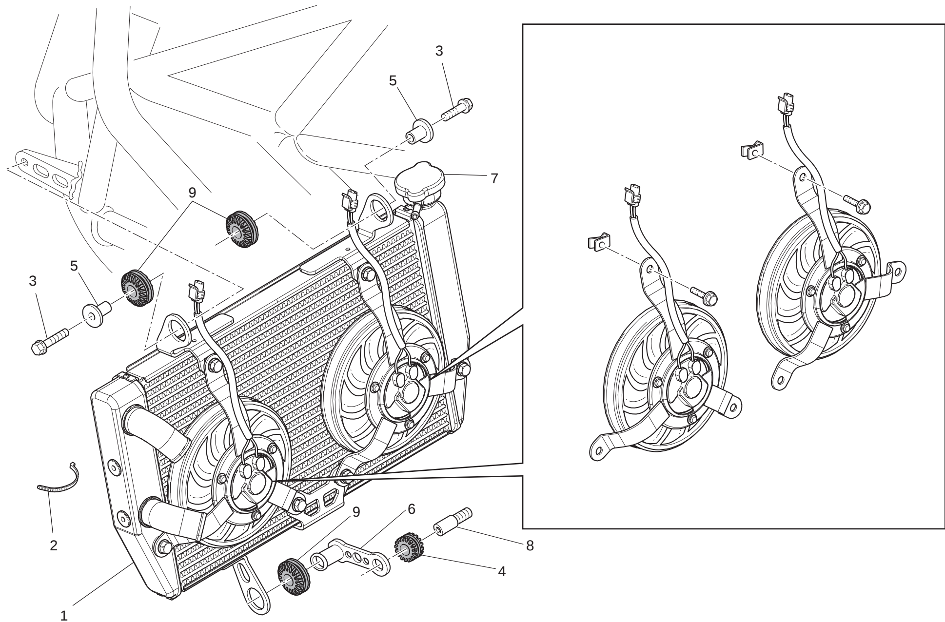
DRAWING 030 Radiator
