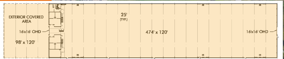
SITE PLAN
