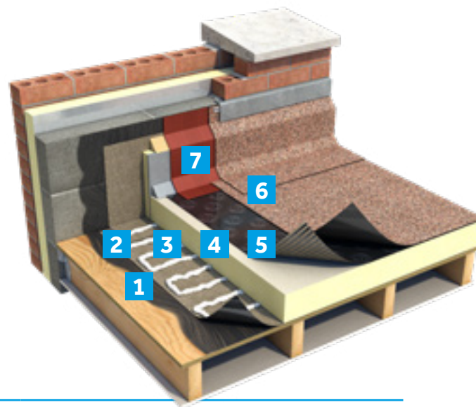
PROFILES XL FIRESMART PLUS: OSB OR PLY SUBSTRATE
