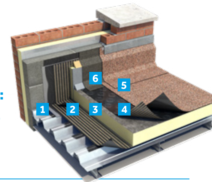
PROFILES XL FIRESMART PLUS: PROFILED METAL SUBSTRATE
