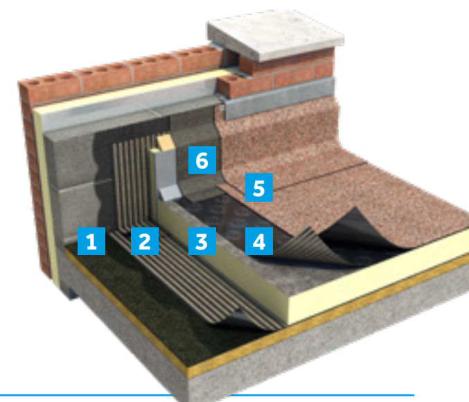
PROFILES XL FIRESMART PLUS: OVERLAY
