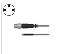
MFS02-S-KHC-P1-PNP Magnetic field sensor Straight Cable 0,3 m - Connector M8
