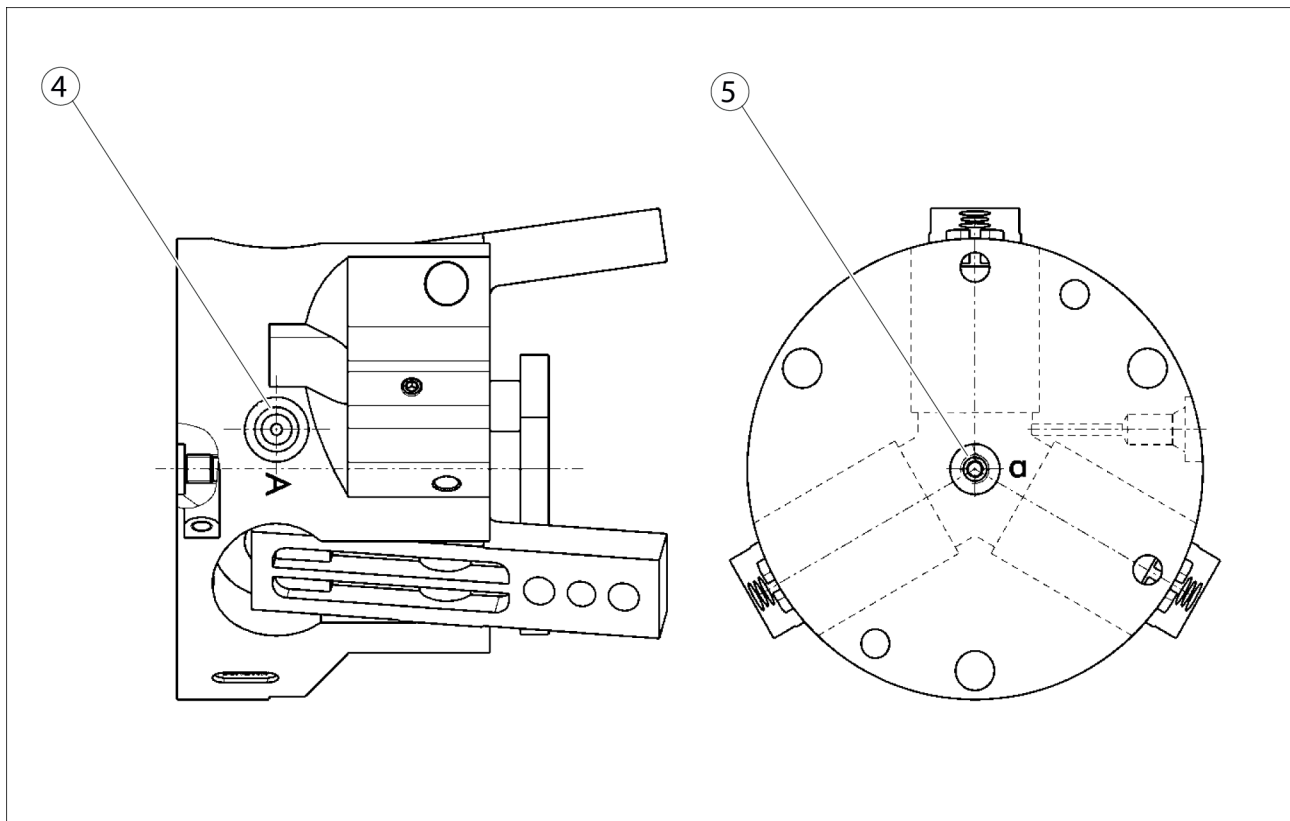
Air connections
