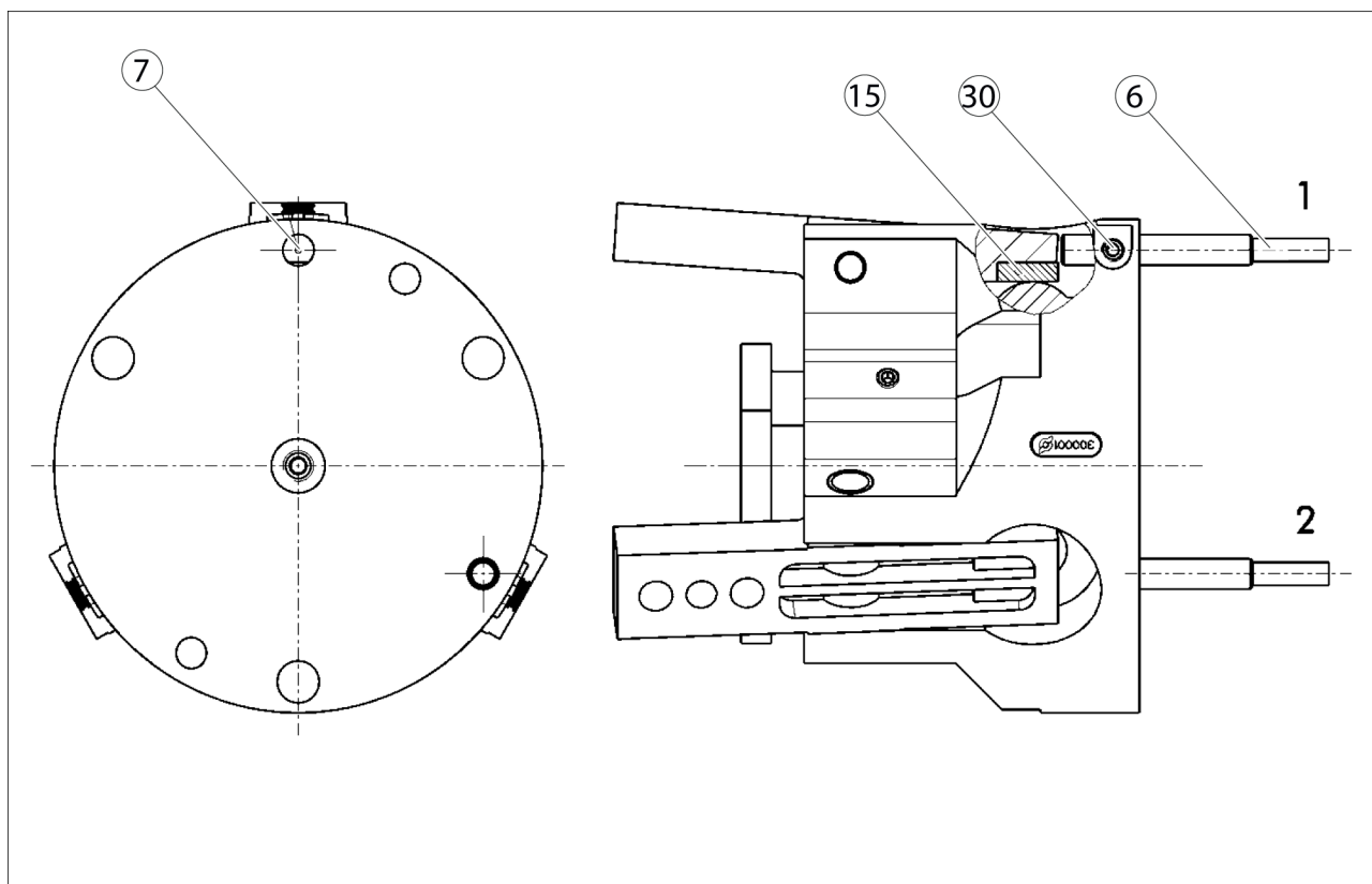
Adjustment inductive proximity switch
