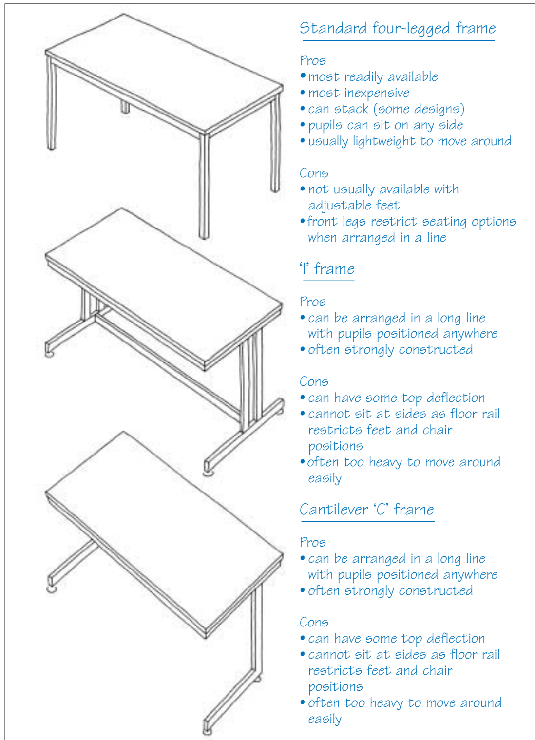
Fig A/1-2: General and Specialist Table Frame Types and their Advantages and Disadvantages.
