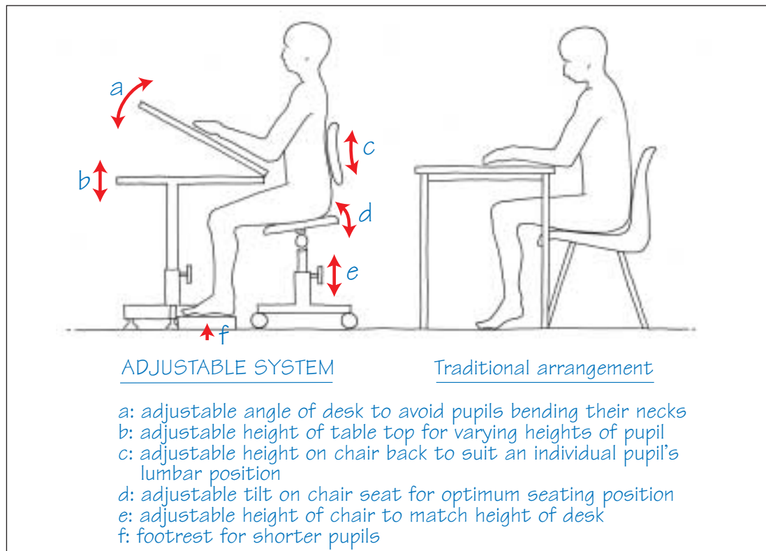
Fig A/2-2: General Principles of Adjustable Height Furniture Systems
