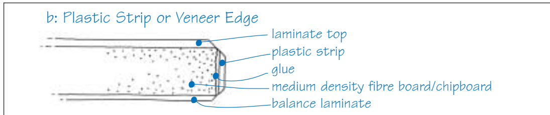
Fig A/3-1b: Plastic Strip or Veneer Edge
