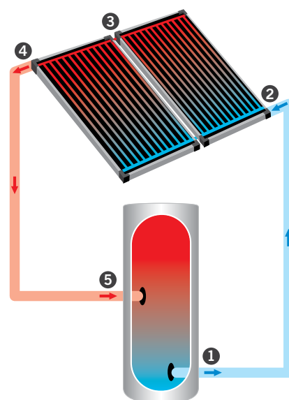
HEATING PROCESS OF WATER TO / FROM TANK AND SOLAR COLLECTORS
