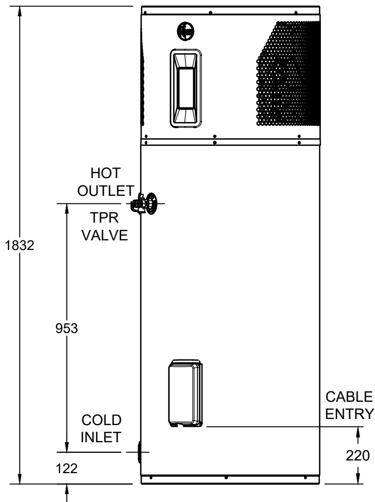
DIMENSIONS AMBIPOWER 280 (551E280) HEAT PUMP WATER HEATER
