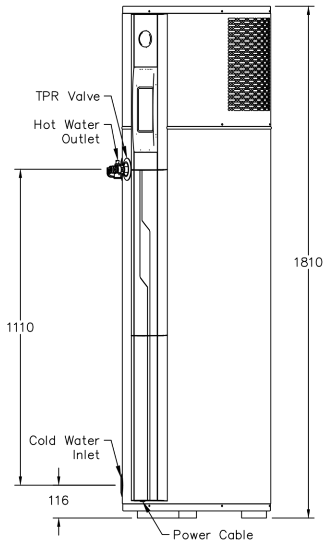
DIMENSIONS 551D180 HEAT PUMP WATER HEATER
