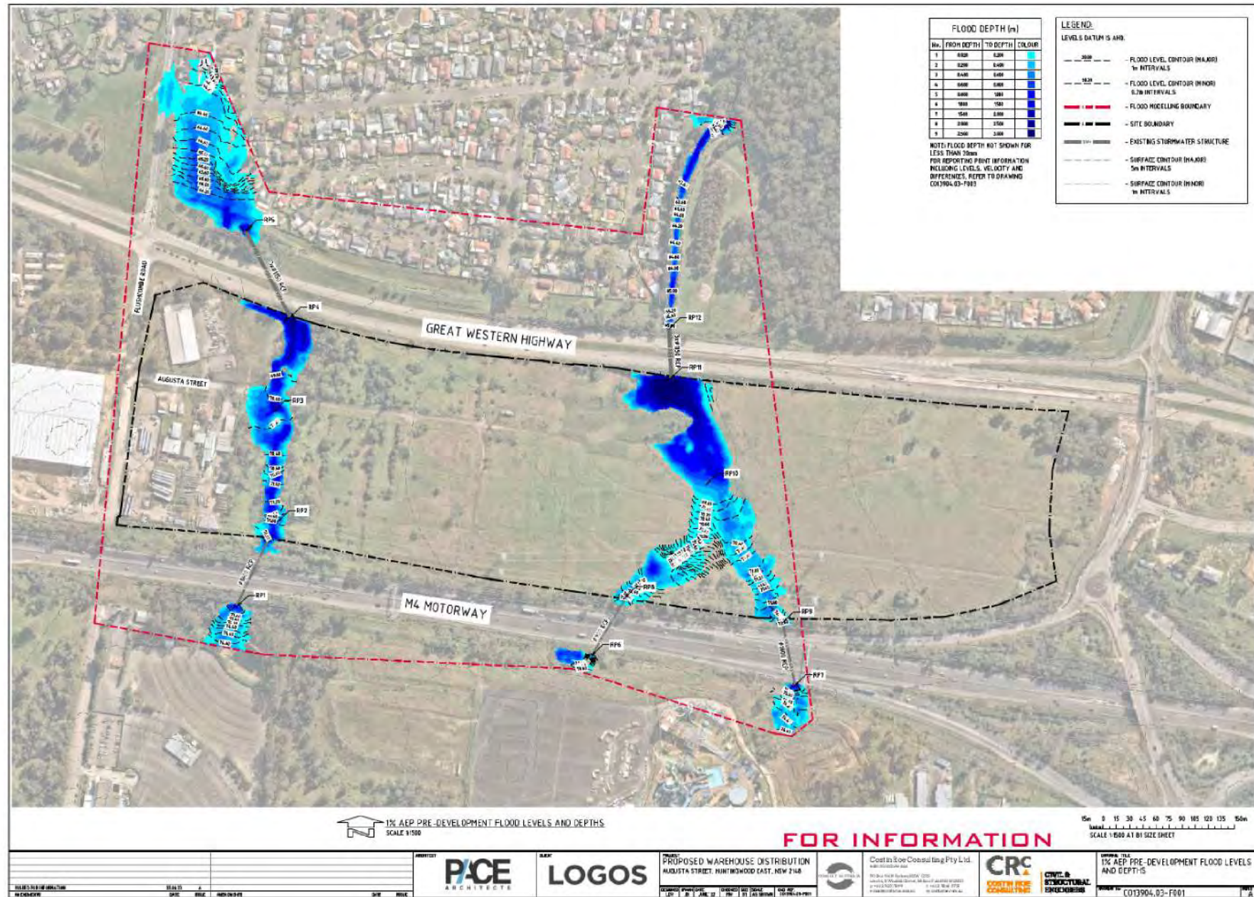
Figure 1e. 1% AEP pre-development flood levels and depth (Costin Roe Consulting Pty Ltd, Drawing No. C013904.03-F001. Issue A. Dated 23.06.23)
