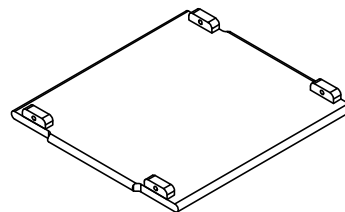
3) Shelf (19.5 x 17.8 x 1.5") x 1 or (49.6 x 45.1 x 3.8 cm)
