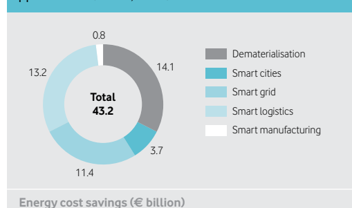
Figure 8. Total cost saving potential for all modelled opportunities (EU-25; 2020)
