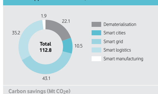
Figure 7. Total carbon abatement potential for all modelled opportunities (EU-25; 2020)
