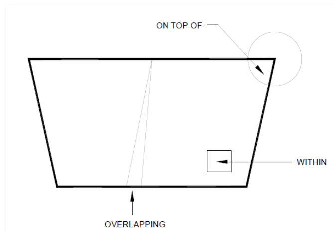
Figure 25. Overlapping Polygons of the Same Feature Type (source: FAA AC150/5300-18B, Change 1)
