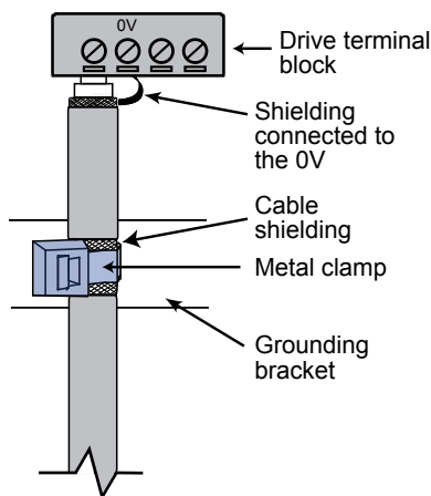
Connecting a control cable to the drive
