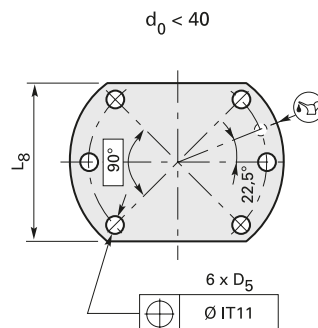
Drilling pattern 1
