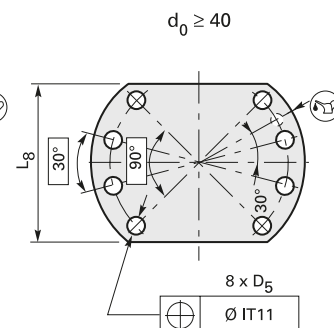
Drilling pattern 1
