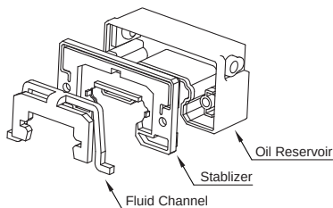
Fig 2.2.14 Cassette Unit
