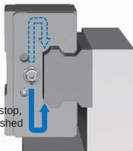
Fig 2.2.10 The oil flows downward through optional screw in spot when the feeding stops
