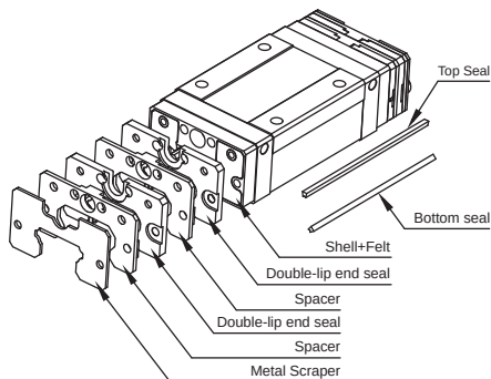
WZ (Two Double-lip end seals+Bottom seals+Top Seals+Felts)
