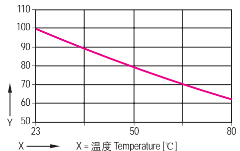
Y = 抗拉强度百分比 Percentage tensile strength [%] 温度对塑料关节轴承的最大抗拉强度的影响 Trends indicate the effect of temperature on the max. load capacity of CSB-BAL® bearings
