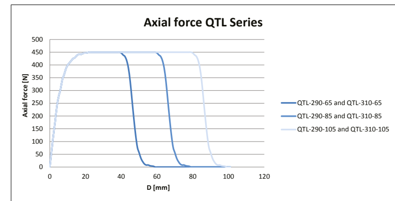
Figure 35: Axial forces QTL 290 and QTL 310 series
