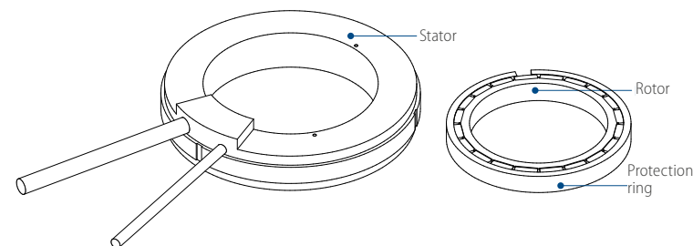
Figure 3: Protection ring
