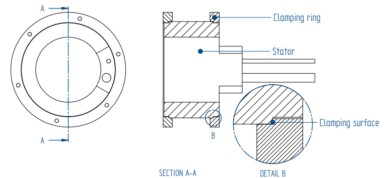
Figure 44: Example clamping ring
