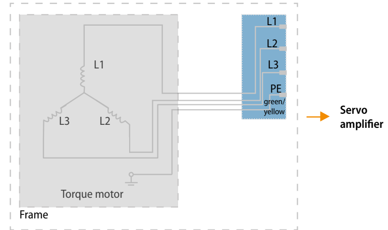
Figure 13: Wiring scheme for QTR 65 and QTR 78
