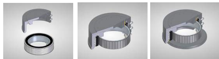
Figure 50: Installation of QTL 230 & 310 motor assembly
