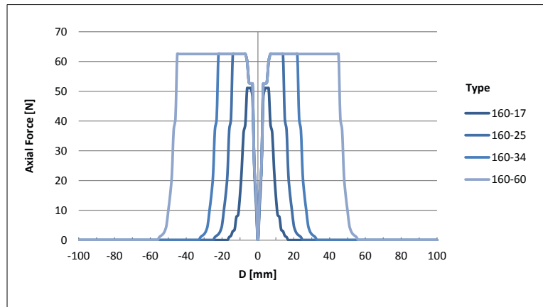
Figure 33: Axial forces QTR 160 series
