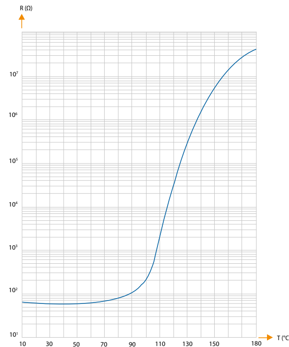
Figure 17: Temperature dependence of the PTC-1k sensor
