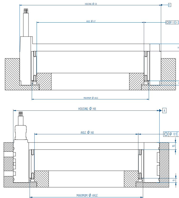
Figure 11: QTL 210 and 290 (above) and 230 and 310 (below) housing requirement tolerances for mounting/centering purposes
