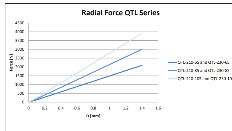
Figure 42: Radial forces QTL 210 and QTL 230 series
