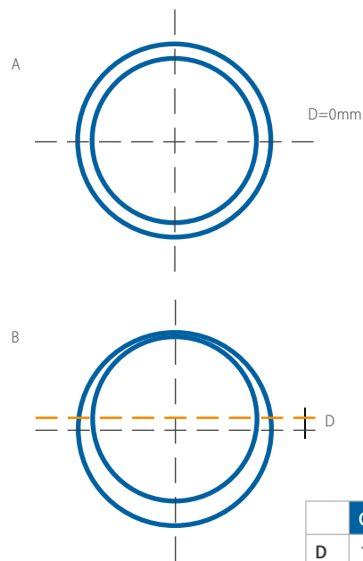
Figure 36: Behaviour of radial attraction forces A - Radial forces in equilibrium B - Radial forces are maximal
