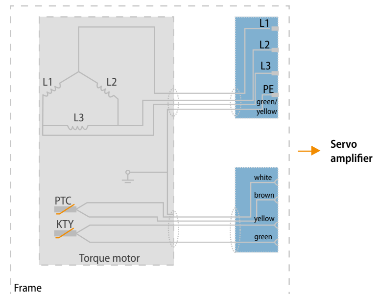
Figure 15: Wiring scheme for torque Z windings
