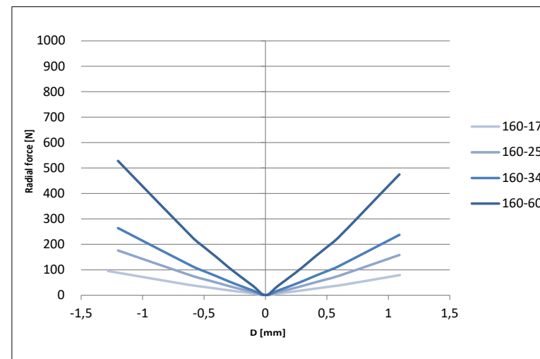
Figure 41: Radial forces QTR160 series
