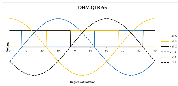
Figure 23: Timing diagram of QTR 65 series
