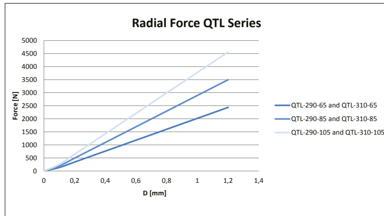
Figure 43: Radial forces QTL 290 and QTL 310 series
