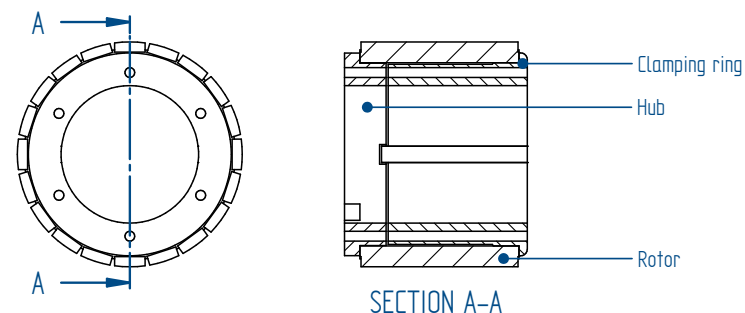
Figure 45: Example clamping ring
