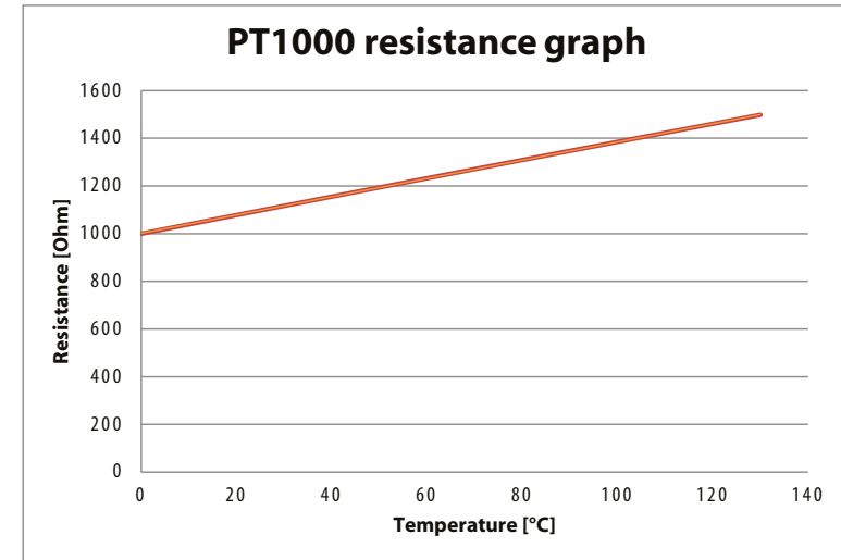
Figure 20: PT 1000 sensor characteristics
