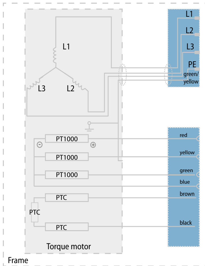
Figure 16: Wiring scheme for QTL series
