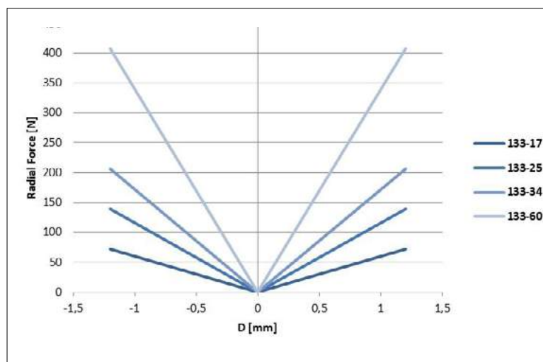
Figure 40: Radial forces QTR133 series
