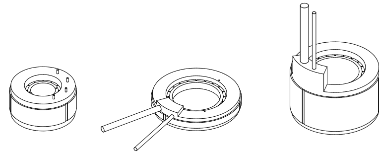
Figure 12: Axial flying lead (left), radial shielded cables (middle), axial shielded cables (right)
