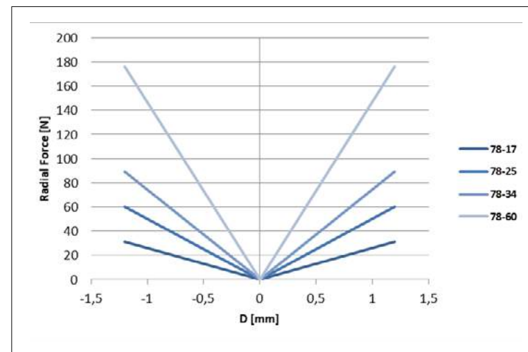
Figure 38: Radial forces QTR 78 series
