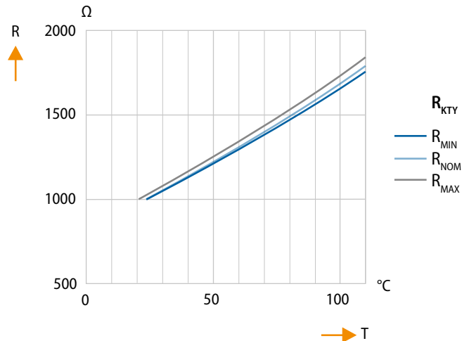
Figure 18: Temperature dependence of the KTY83-122 sensor
