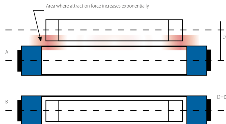
Figure 28: Behaviour of axial attraction forces
