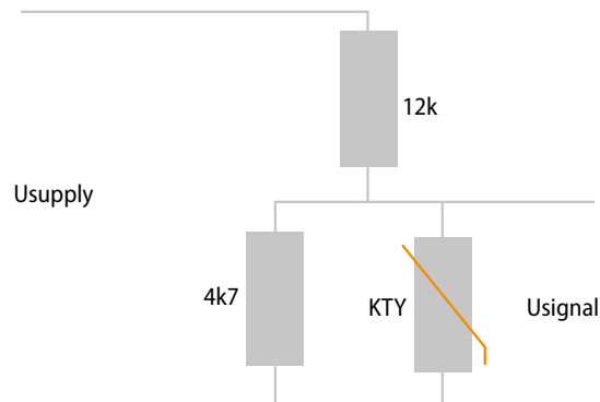
Figure 19: Wiring scheme for KTY83-122 sensor
