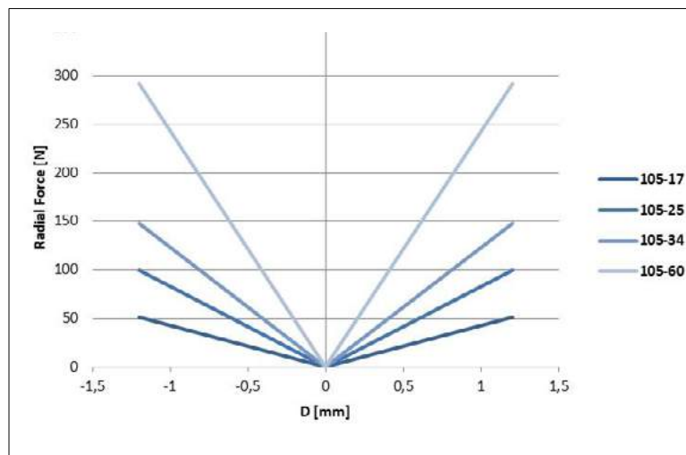
Figure 39: Radial forces QTR105 series
