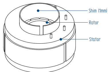
Figure 47: Rotor and stator packaging of QTR 65 and QTR 78
