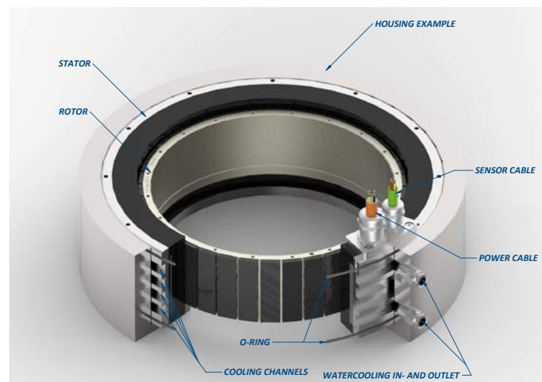
Figure 7: Material overview of QTL 230 and QTL 310 with O-rings
