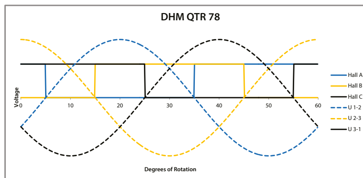
Figure 24: Timing diagram of QTR 78 series
