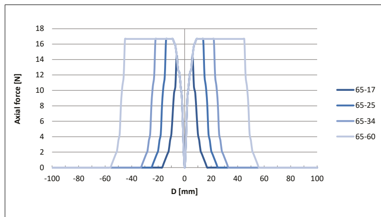
Figure 29: Axial forces QTR 65 series
