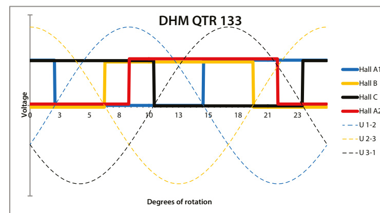
Figure 26: Timing diagram of QTR 133 series
