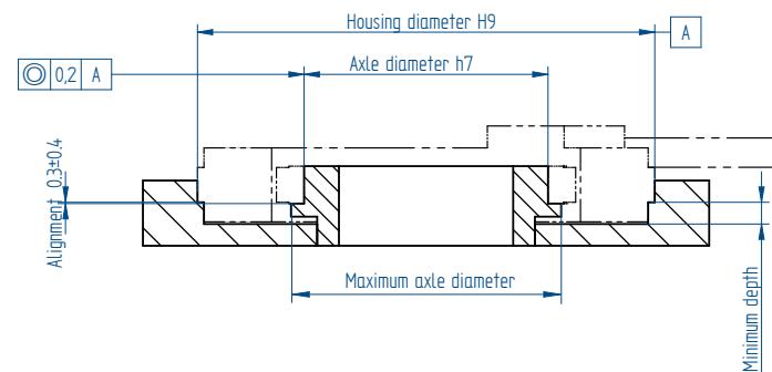
Figure 10: QTR 1xx housing requirement tolerances for mounting/centering purposes
