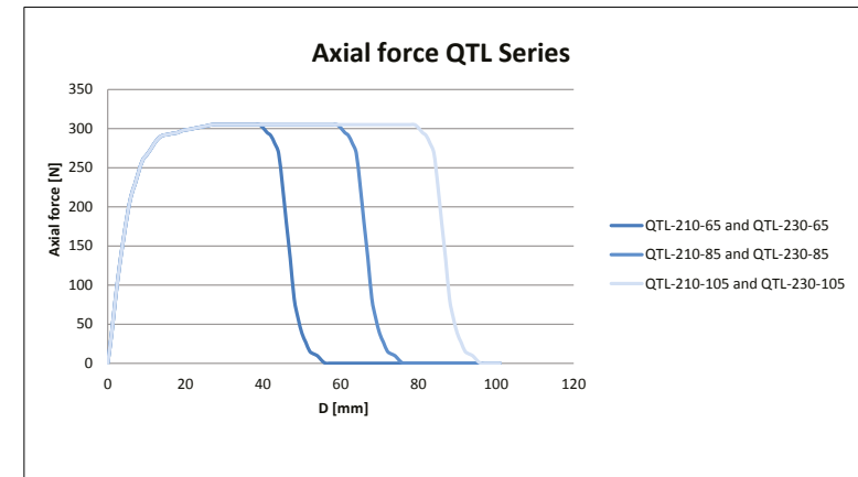
Figure 34: Axial forces QTL 210 and QTL 230 series
