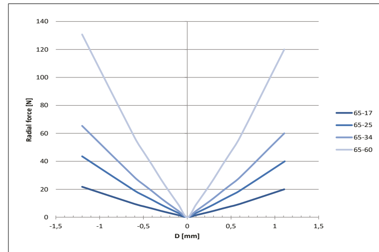
Figure 37: Radial forces QTR 65 series
