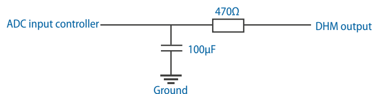
Figure 21: Output filter
