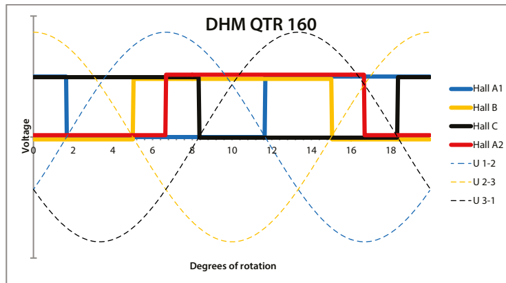
Figure 27: Timing diagram of QTR 160 series
