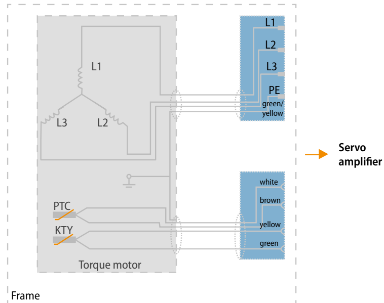
Figure 14: Wiring scheme for QTR 105, QTR 133 and QTR 160
