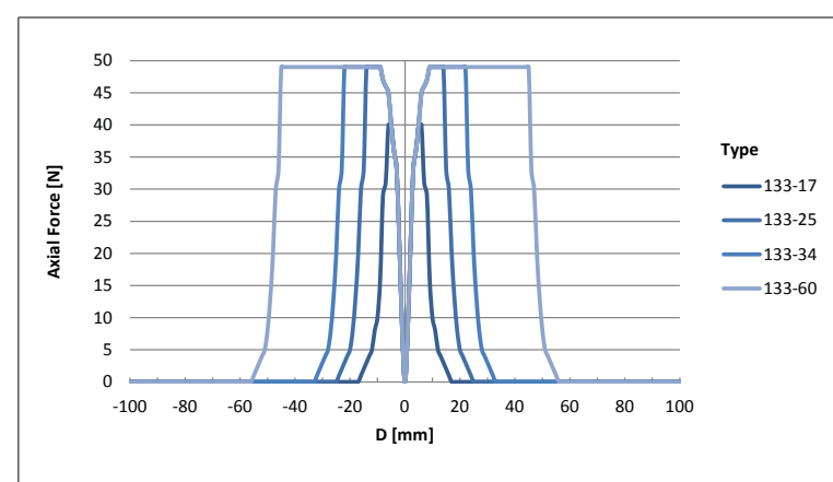
Figure 32: Axial forces QTR 133 series
