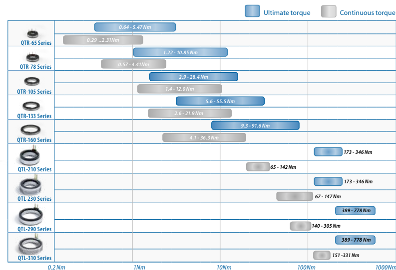
Figure 1: Torque range
