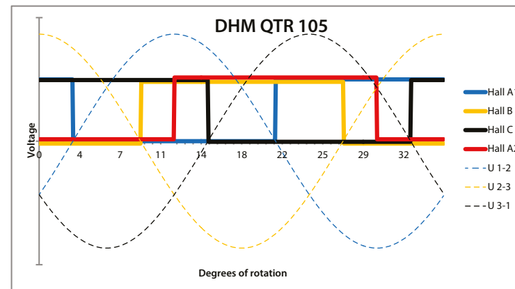
Figure 25: Timing diagram of QTR 105 series
