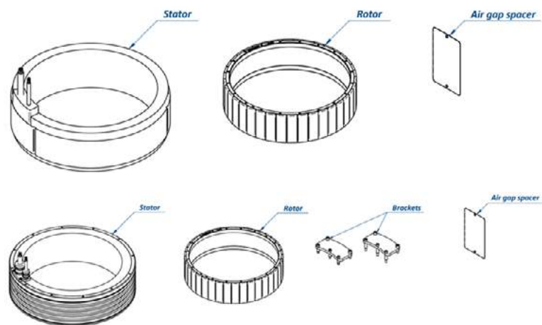
Figure 2: Basic components QTL motor kit
