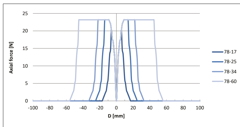
Figure 30: Axial forces QTR 78 series
