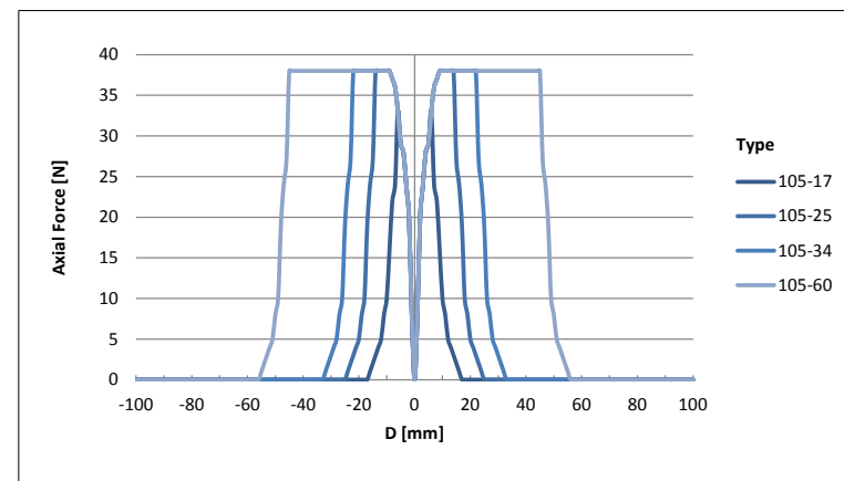
Figure 31: Axial forces QTR 105 series
