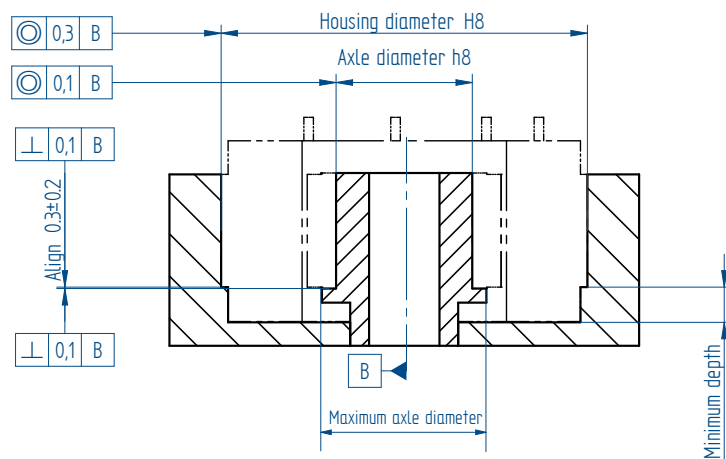
Figure 9: QTR 65 and QTR 78 housing requirement tolerances for mounting/centering purposes
