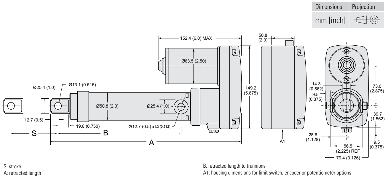
Stroke, Retracted Length and Weight Relationships
