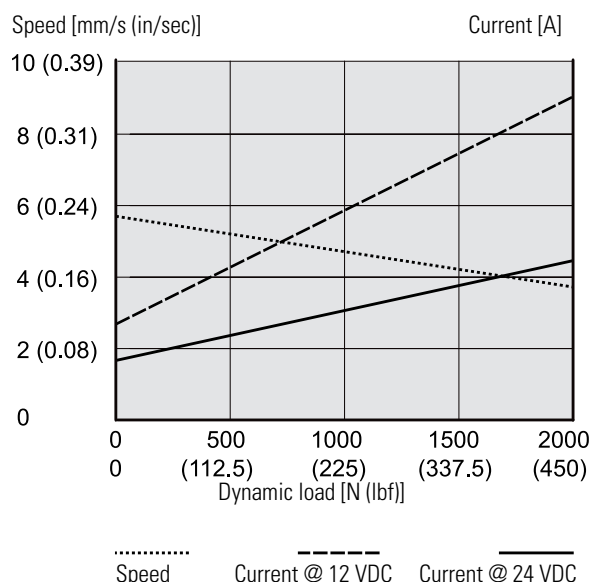
Speed and Current vs. Load
