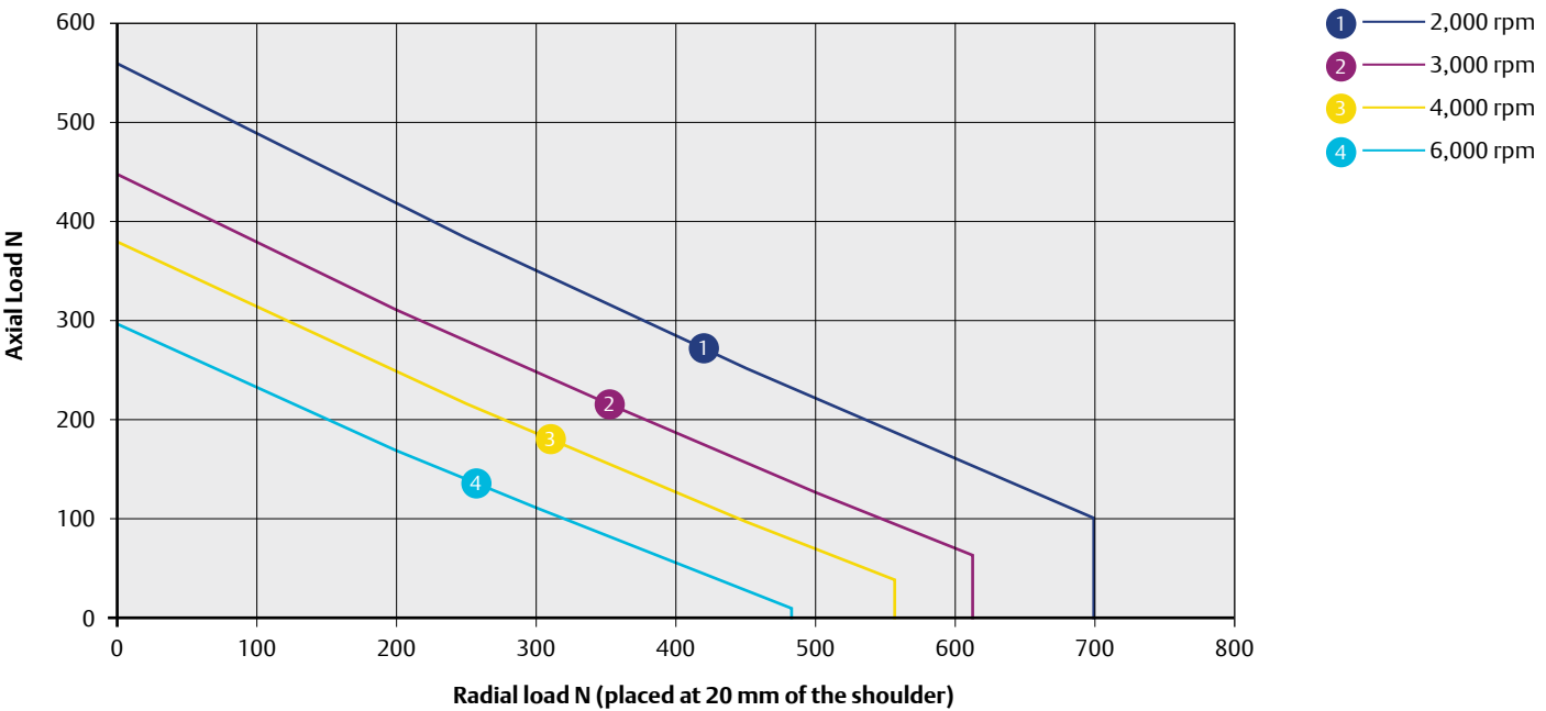
Radial load vs. axial load on 067UD/ED
