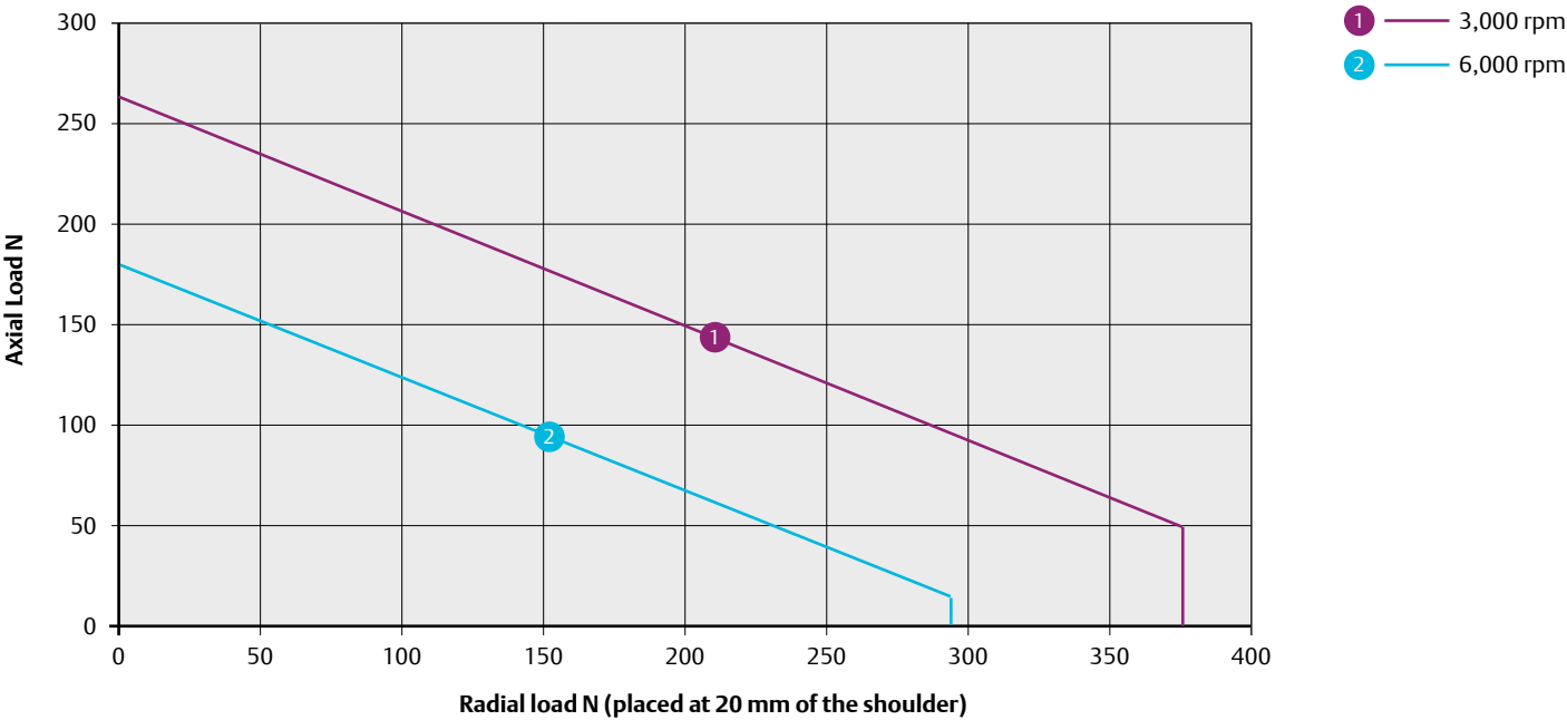
Radial load vs. axial load on 055UD/ED
