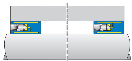
This ETP-AXPRESS is used for fastening and centering of a cylinder in a printing machine for beverage cans of aluminium. It has two separate pressure chambers, one for expansion to the shaft and one to the bore of the cylinder. The runout is better and downtime much shorter than with the mechanical clamping used before
