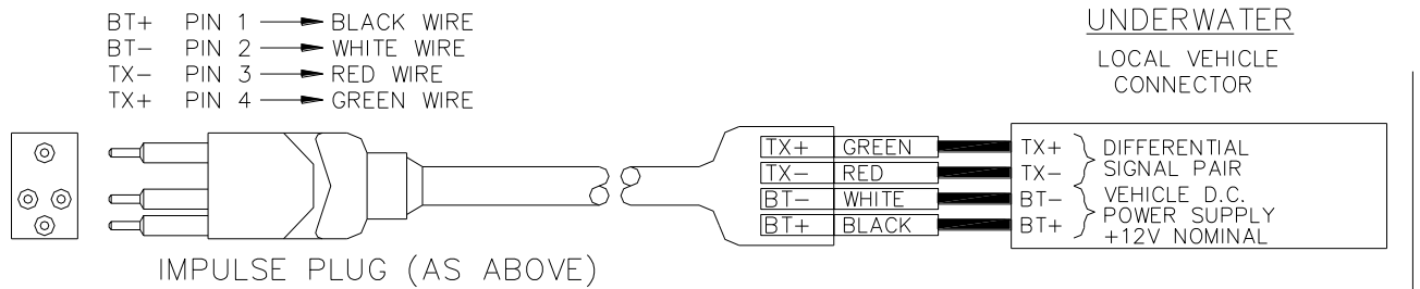
CONNECTION DIAGRAM FOR EITHER OPTION
