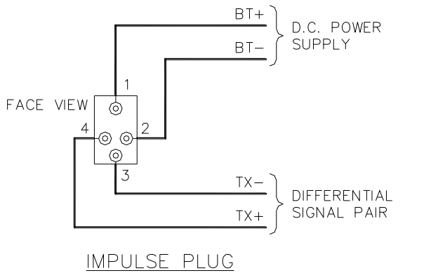
CONNECTION DIAGRAM FOR EITHER OPTION
