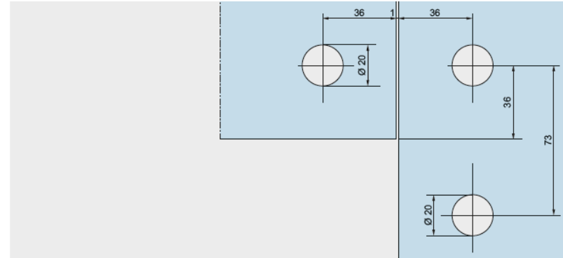
PT 10, PT 20, PT 22, PT 30 Top and bottom patches, overpanel patch
