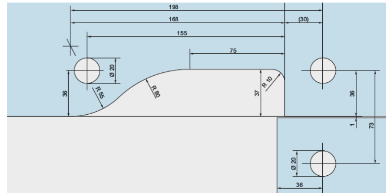
PT 40 Angle patch fitting with continuous overpanel
