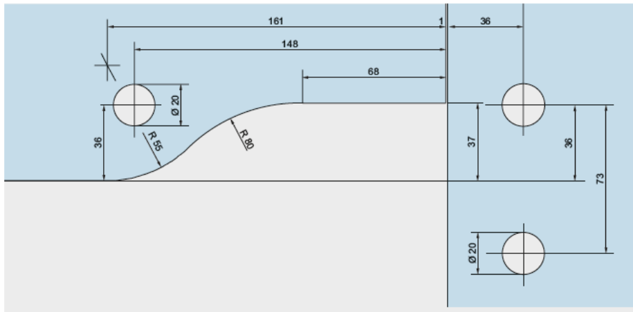
PT 40 Patch for overpanel and sidelight
