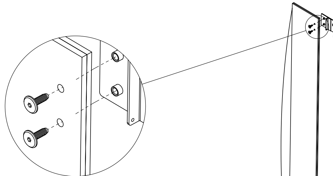
20mmFT DECO BOLT - BB - BLACK 4x
