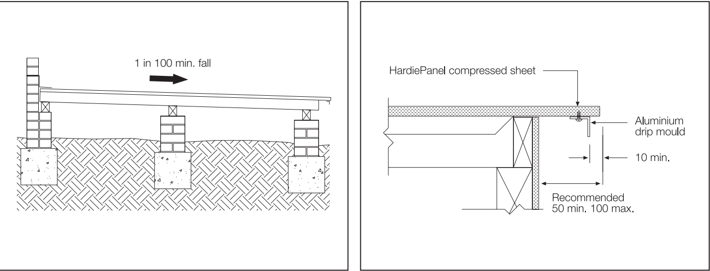
FIGURE 1 FALL FOR DRAINAGE
