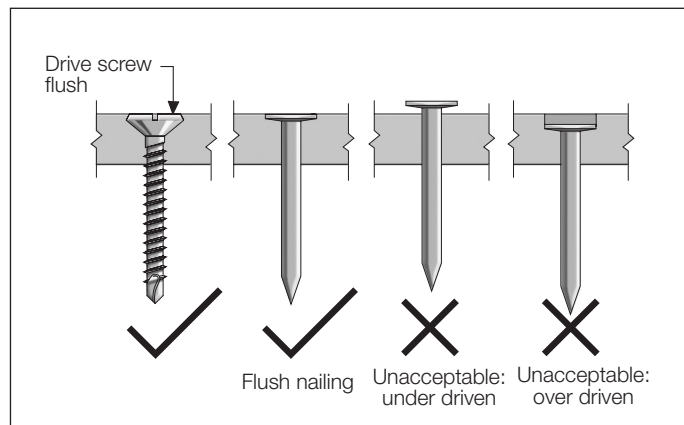
FIGURE 2 FASTENER DEPTH
