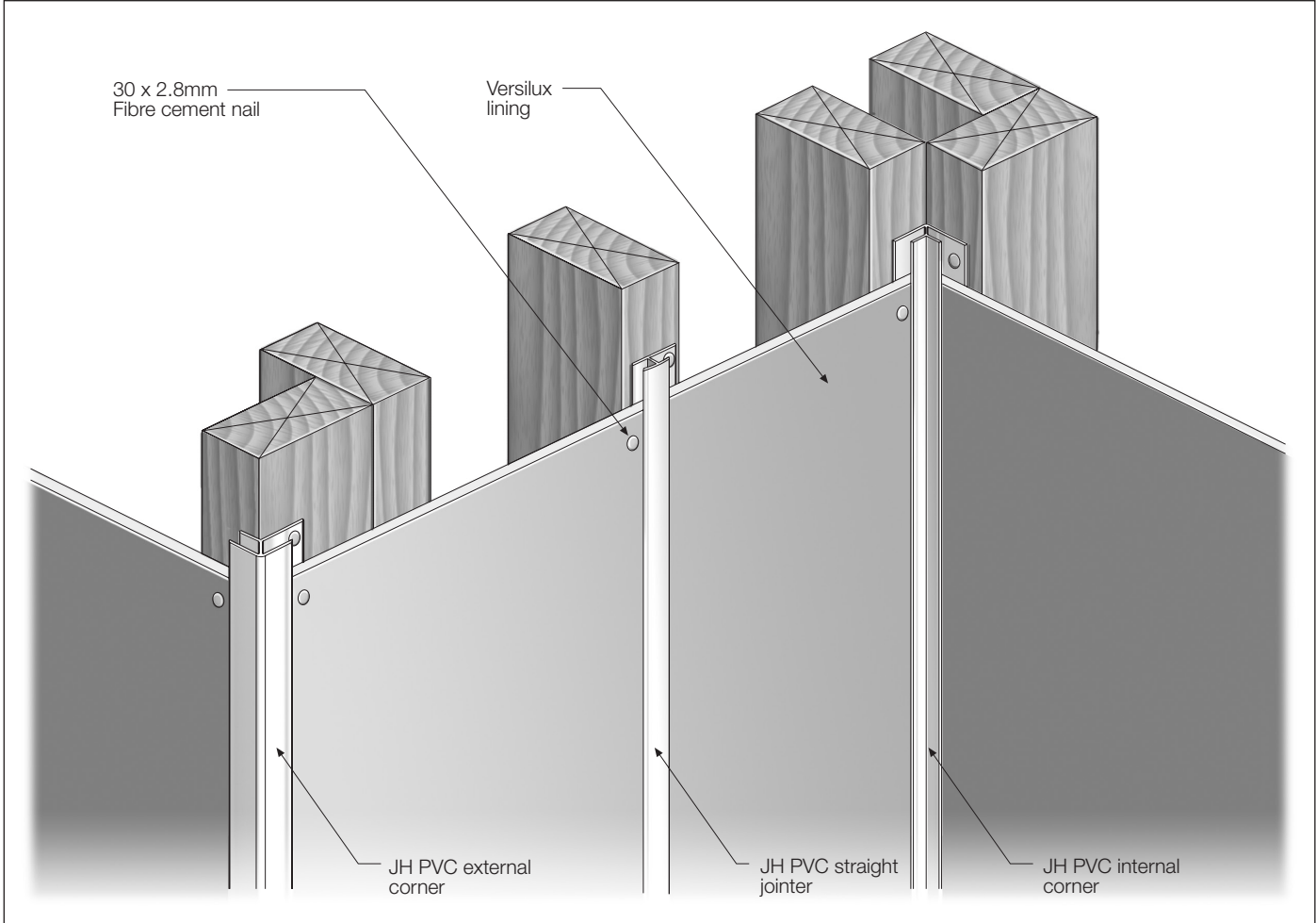
FIGURE 15 CORNER DETAILS
