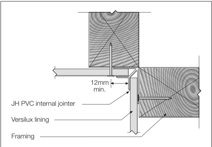
FIGURE 17 INTERNAL CORNER
