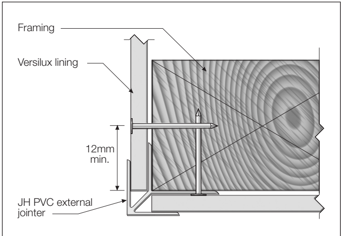
FIGURE 16 EXTERNAL CORNER
