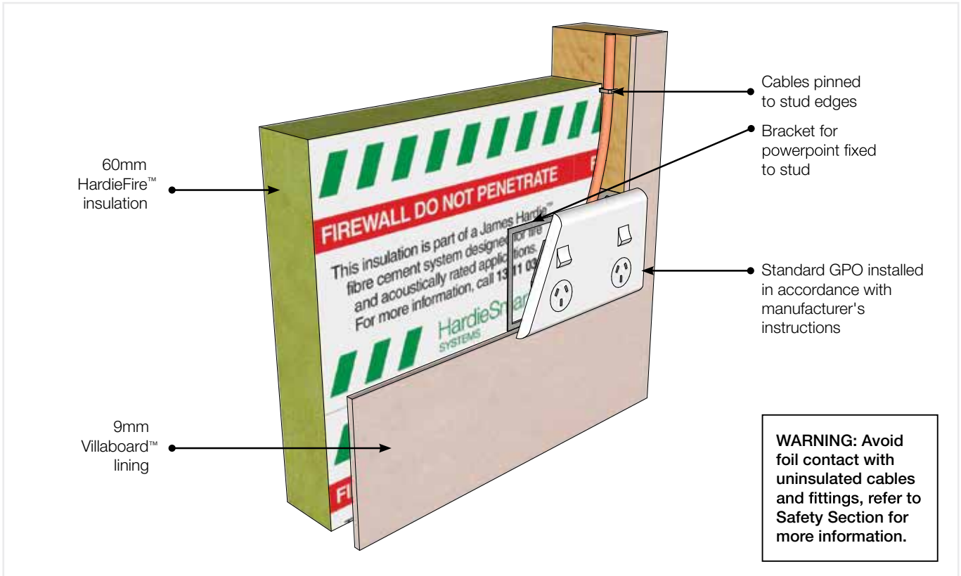
FIGURE 20 ELECTRICAL SERVICES (GPO/POWER POINTS) PERSPECTIVE
