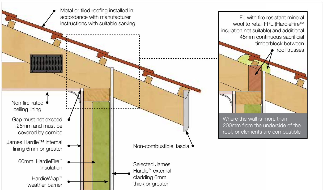
FIGURE 13 EXTERNAL BOUNDARY WALL TO ROOF WITH NO EAVE LINING
