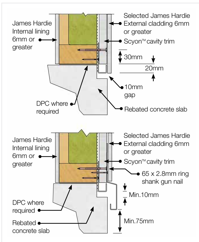
FIGURE 4 SCYON™ CAVITY TRIM SLAB EDGE DETAIL
