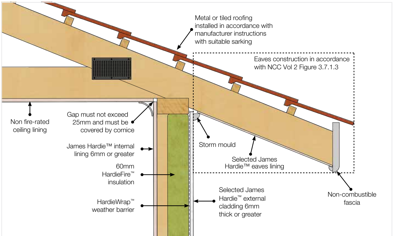
FIGURE 11 EXTERNAL BOUNDARY WALL TO JAMES HARDIE™ EAVE LINING (RAKED) OPTION 2
