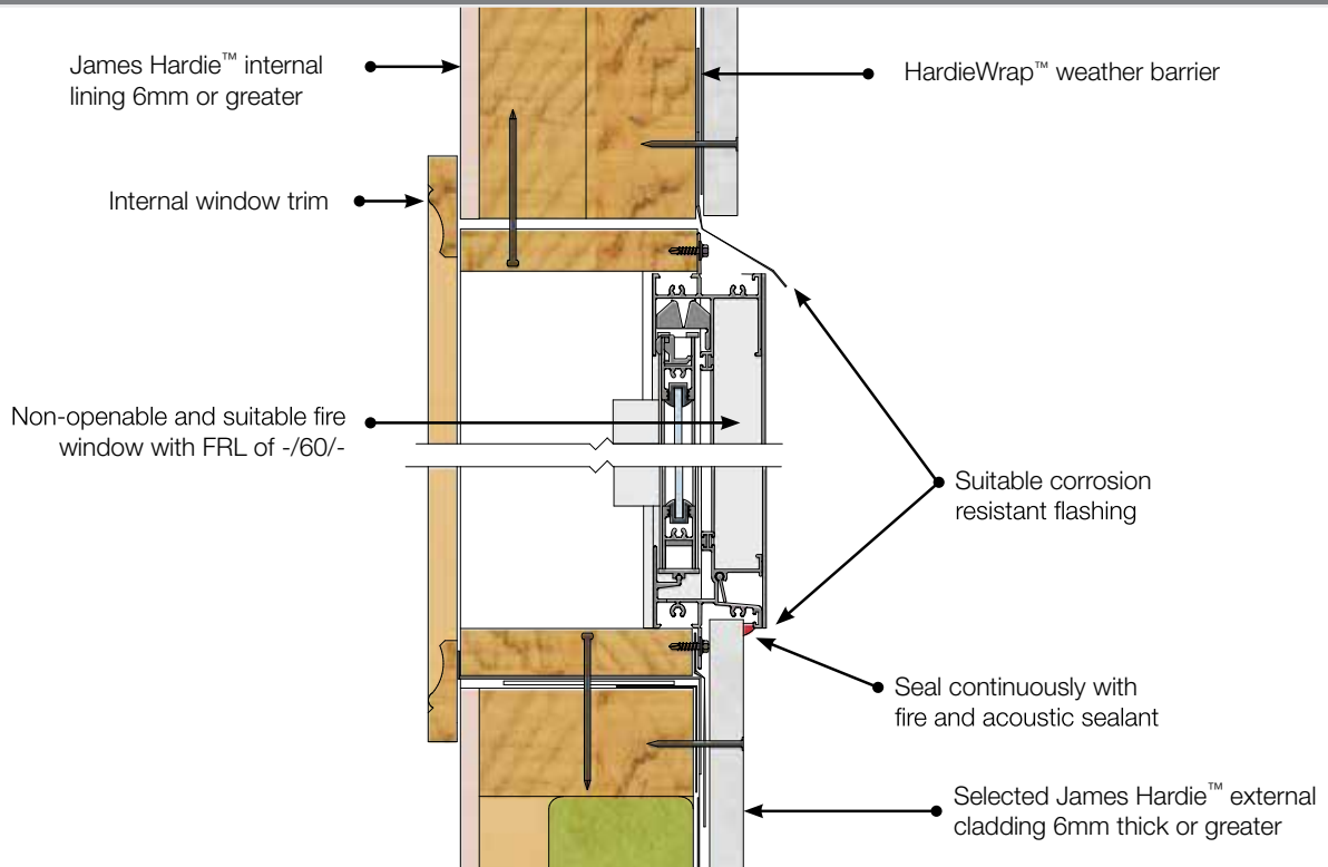
FIGURE 8 FIRE RATED EXTERNAL WINDOW (GUIDE ONLY, PLEASE REFER TO WINDOW MANUFACTURER)
