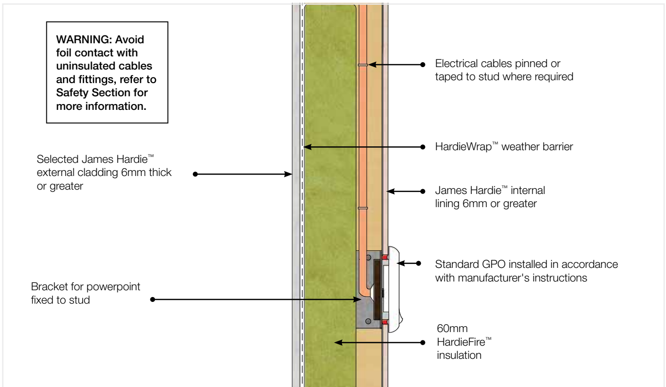
FIGURE 19 ELECTRICAL SERVICES (GPO/POWER POINTS) - SECTION FROM SIDE
