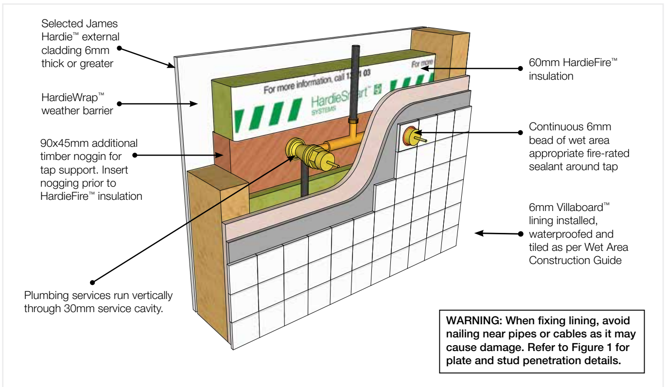
FIGURE 23 HOT/COLD PLUMBING TAPS - PERSPECTIVE
