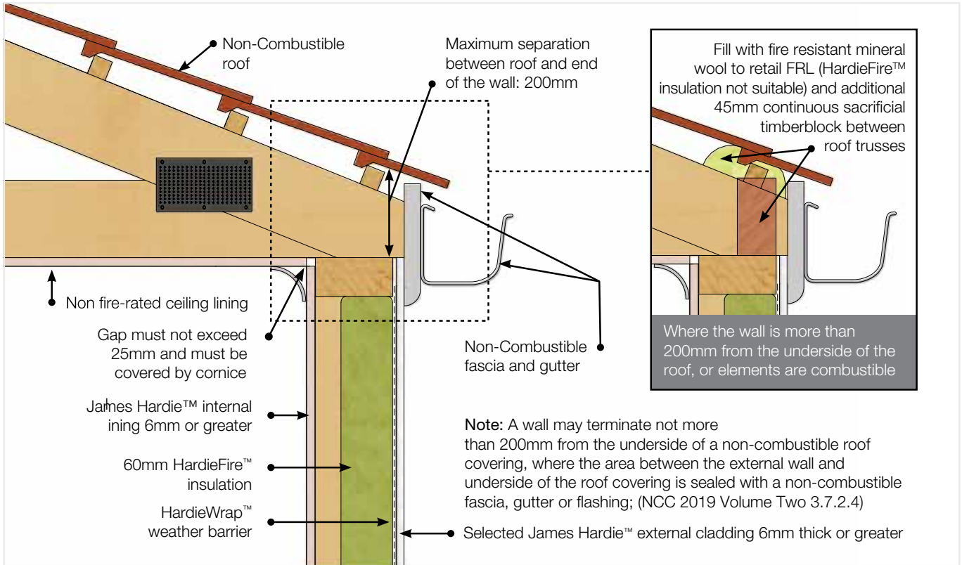
FIGURE 12 EXTERNAL BOUNDARY WALL TO ROOF
