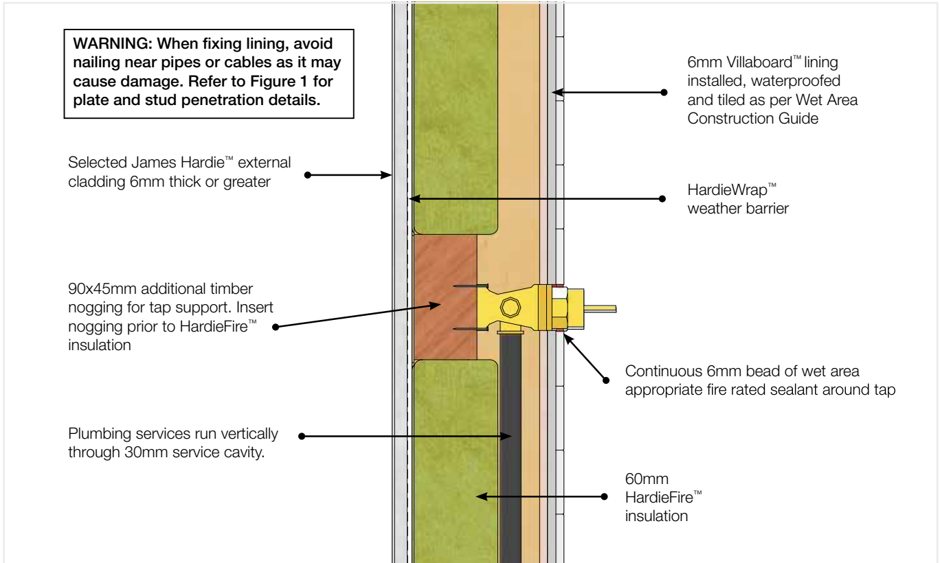
FIGURE 22 HOT/COLD PLUMBING TAPS - SECTION FROM SIDE
