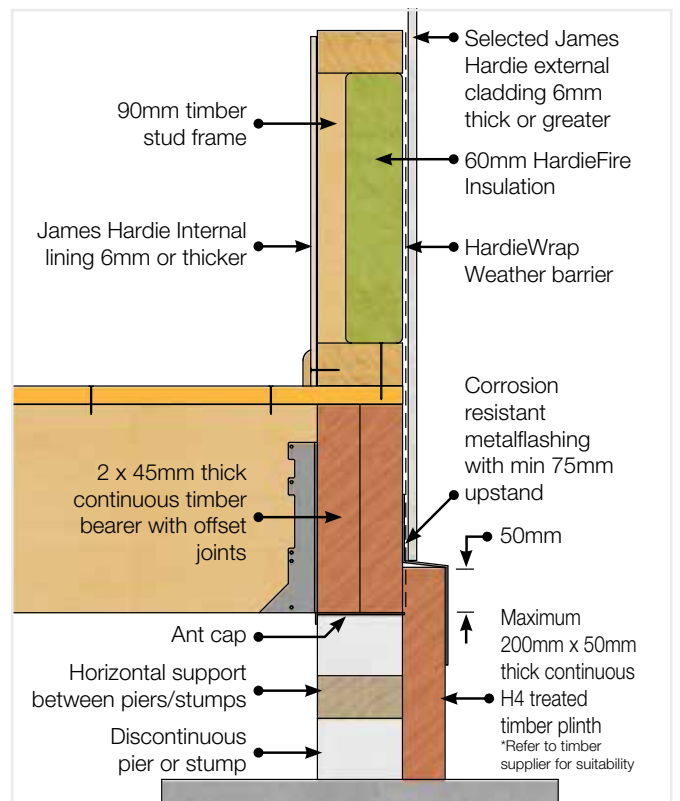
FIGURE 5 PLINTH DETAIL
