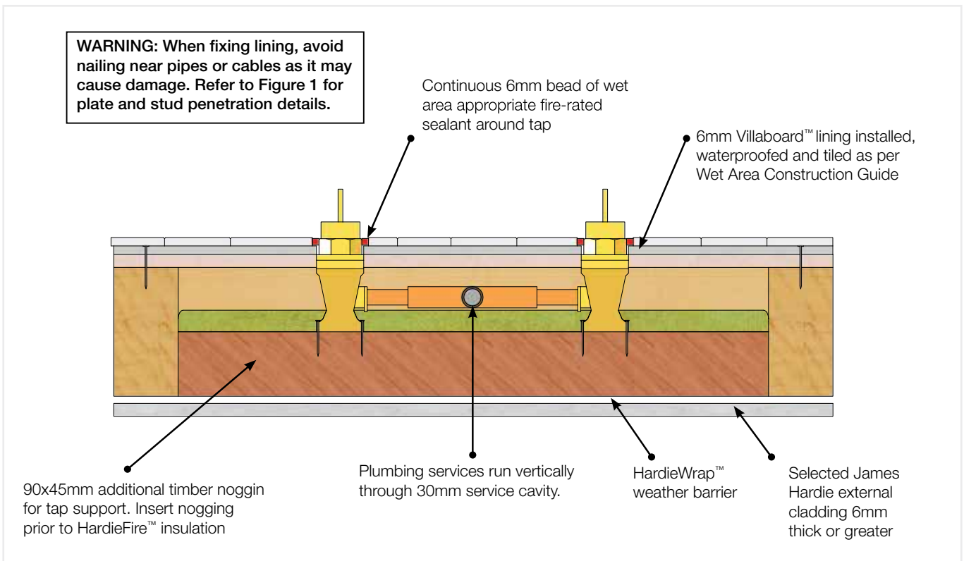
FIGURE 21 HOT/COLD PLUMBING TAPS - SECTION FROM ABOVE
