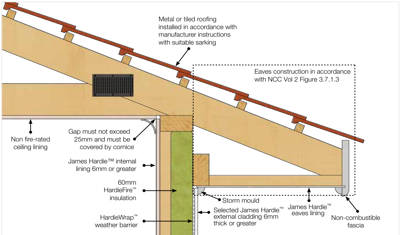
FIGURE 10 EXTERNAL BOUNDARY WALL TO JAMES HARDIE™ EAVE LINING OPTION 1
